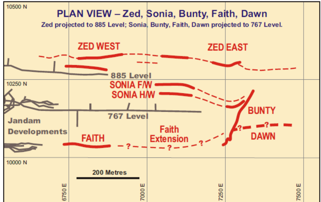
Figure 1: - Plan section showing Faith and Dawn target zones in relation to the Zed Sonia and Bunty orebodies at Pajingo Gold Mine
